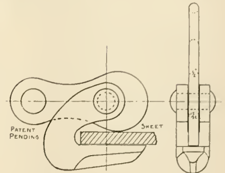
HANDY BOILER PLATE CLIP.
